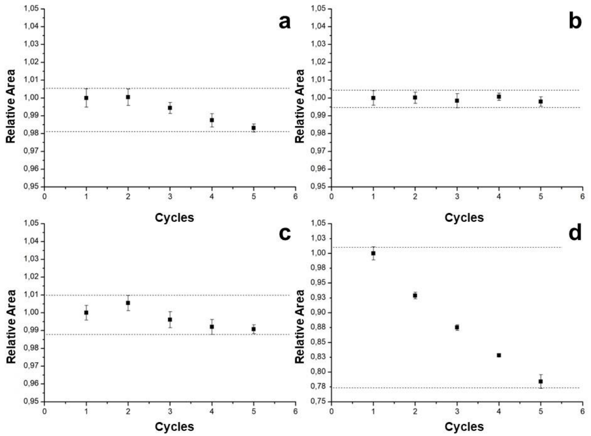
Figure 2. Repeatability for 5 cycles using \beta radiation on (a) TLD-100, (b) TLD-200, (c) TLD-400 and (d) GR-200 dosimeters
